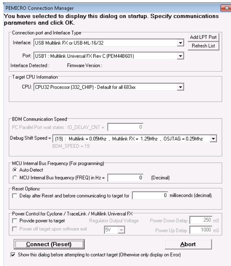
Figure 5-1: Connection Manager Dialog
